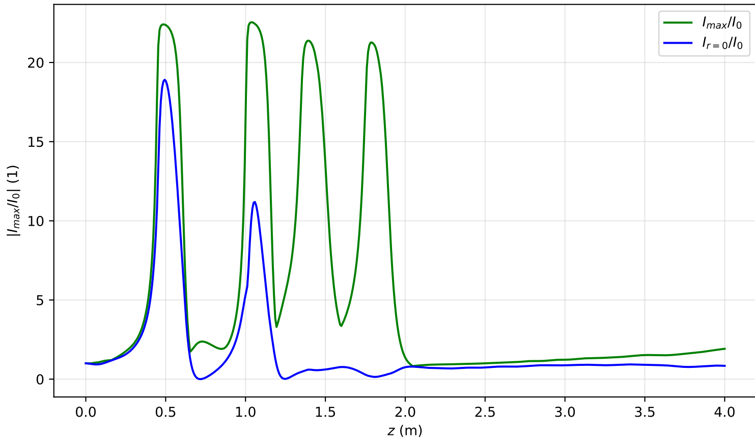
I_{max}(x=0, y=0, z)/I_0 , P_{in}=4.9P_{cr} , noisy input, artificial time
